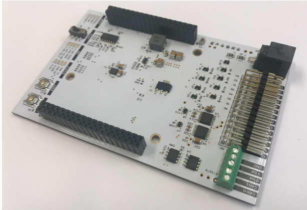
Abbildung 9: ZHAW-Motherboard
